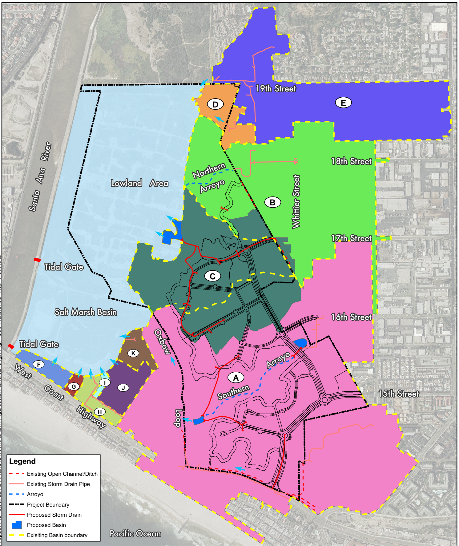
FIGURE 7: Proposed Sub-Watershed Basins
