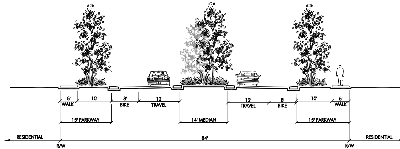
SECTION E-E
