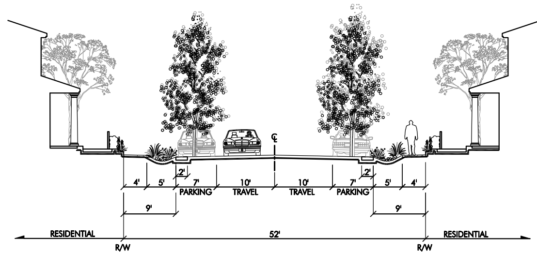
SECTION I-I
