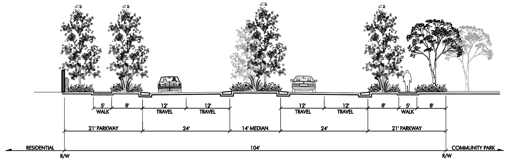
SECTION C-C
