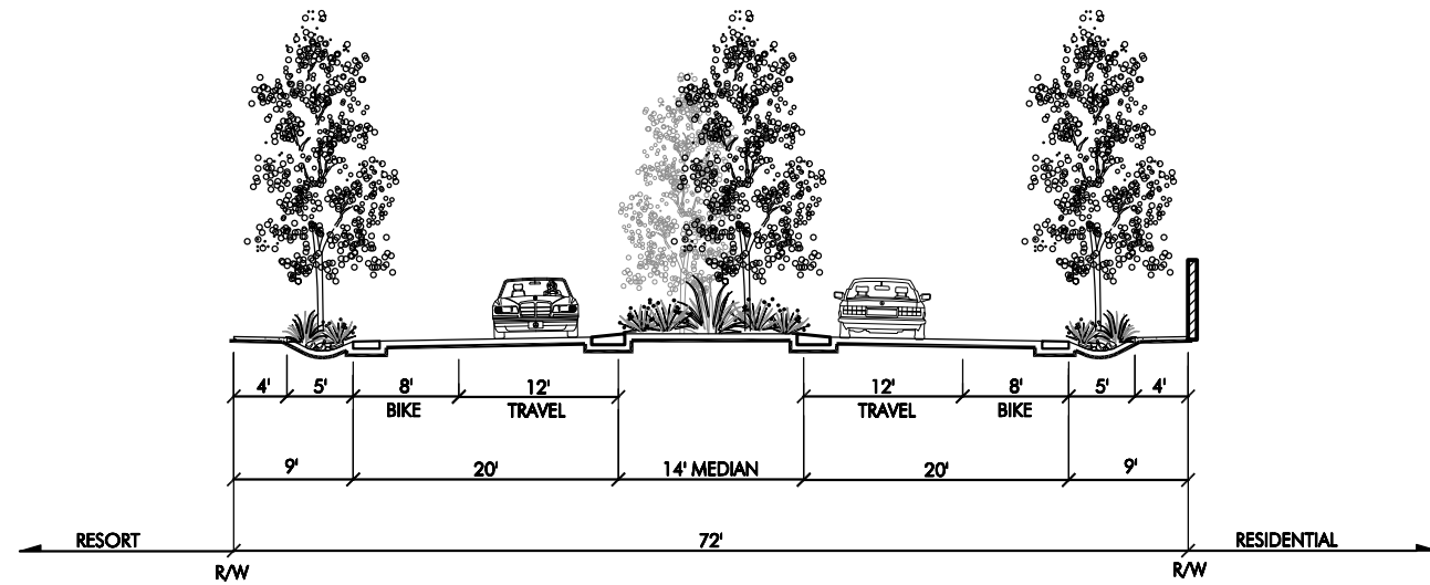
SECTION G-G
