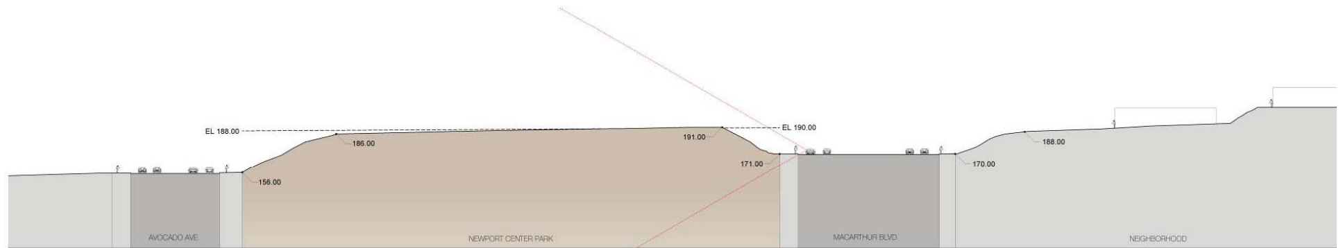
VIEW PROTECTION BY BERM SECTION I
