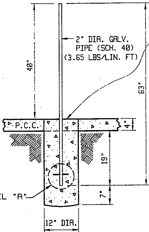
SECTION "X"-"X"
