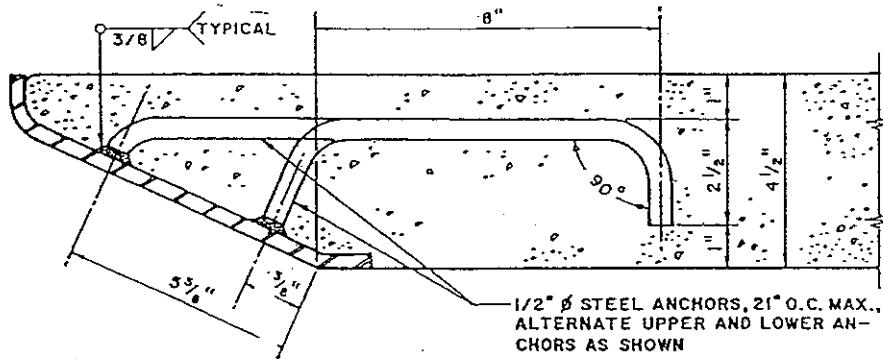
HOOK ANCHOR - 4 1/2" TOP SLAB
