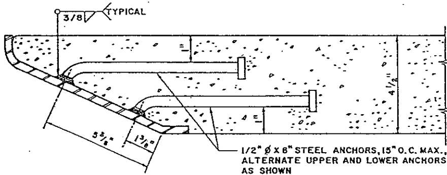
ROUND HEAD ANCHOR - 4 1/2" TOP SLAB
