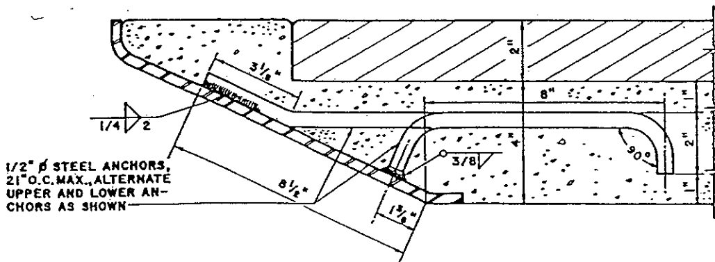
HOOK ANCHOR - 6" TOP SLAB
