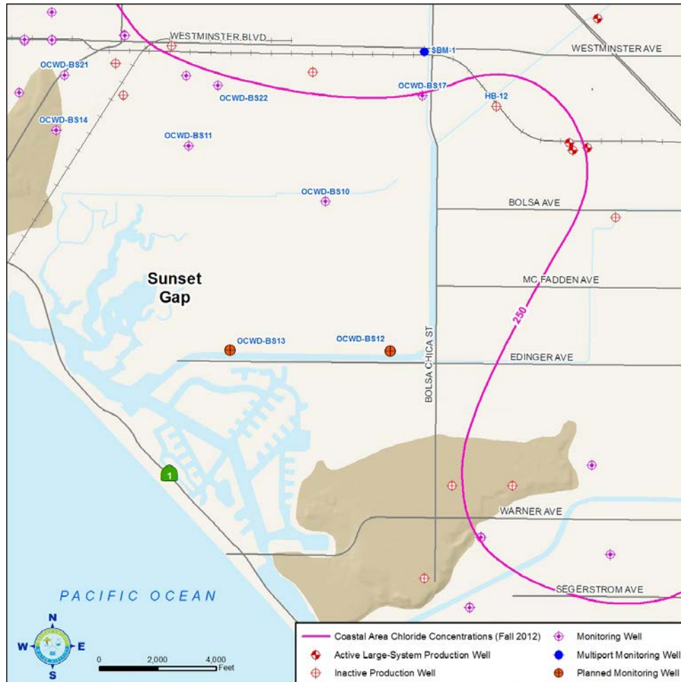
Figure 7-7: Sunset Gap Monitoring and Production Wells with Chloride Concentration Contour
