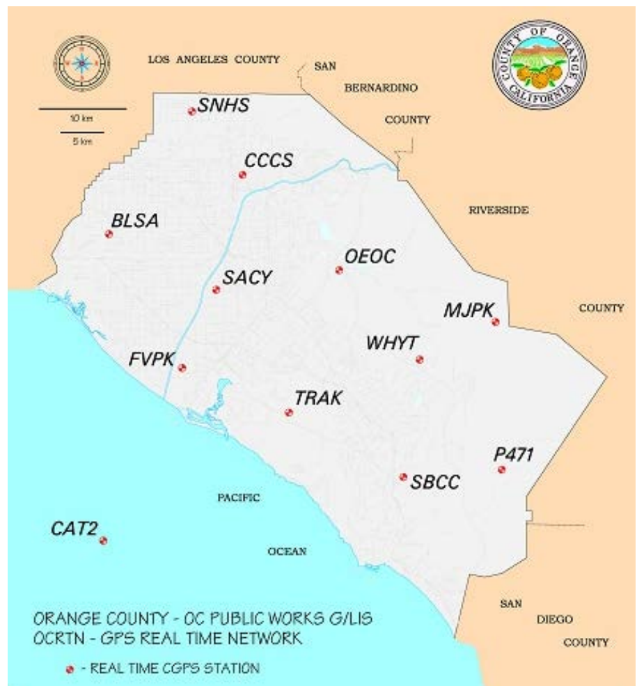
Figure 3-17: Orange County Public Works GPS Real Time Network
