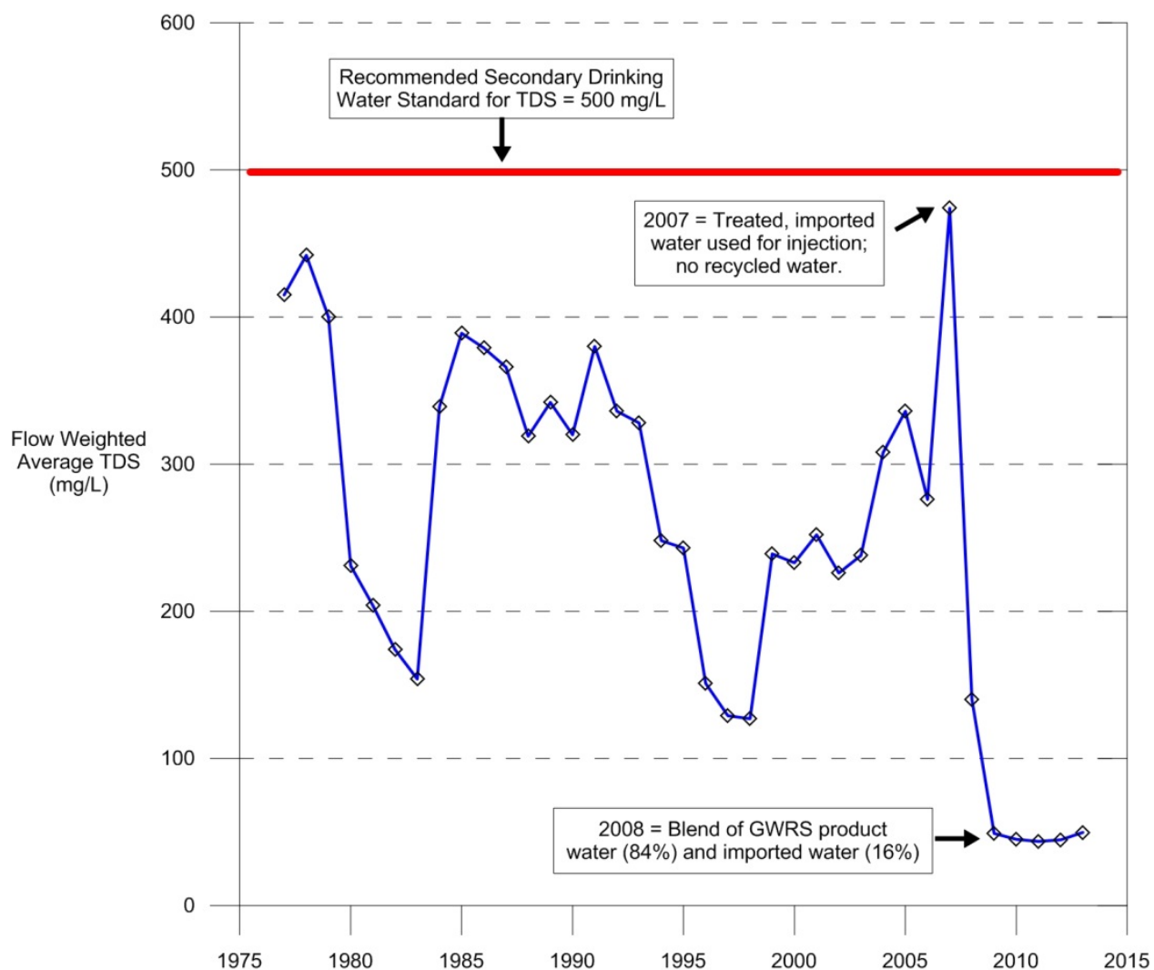
Figure 8-3: Total Flow Weighted Average TDS of All Source Waters Used for Injection at the Talbert Barrier
