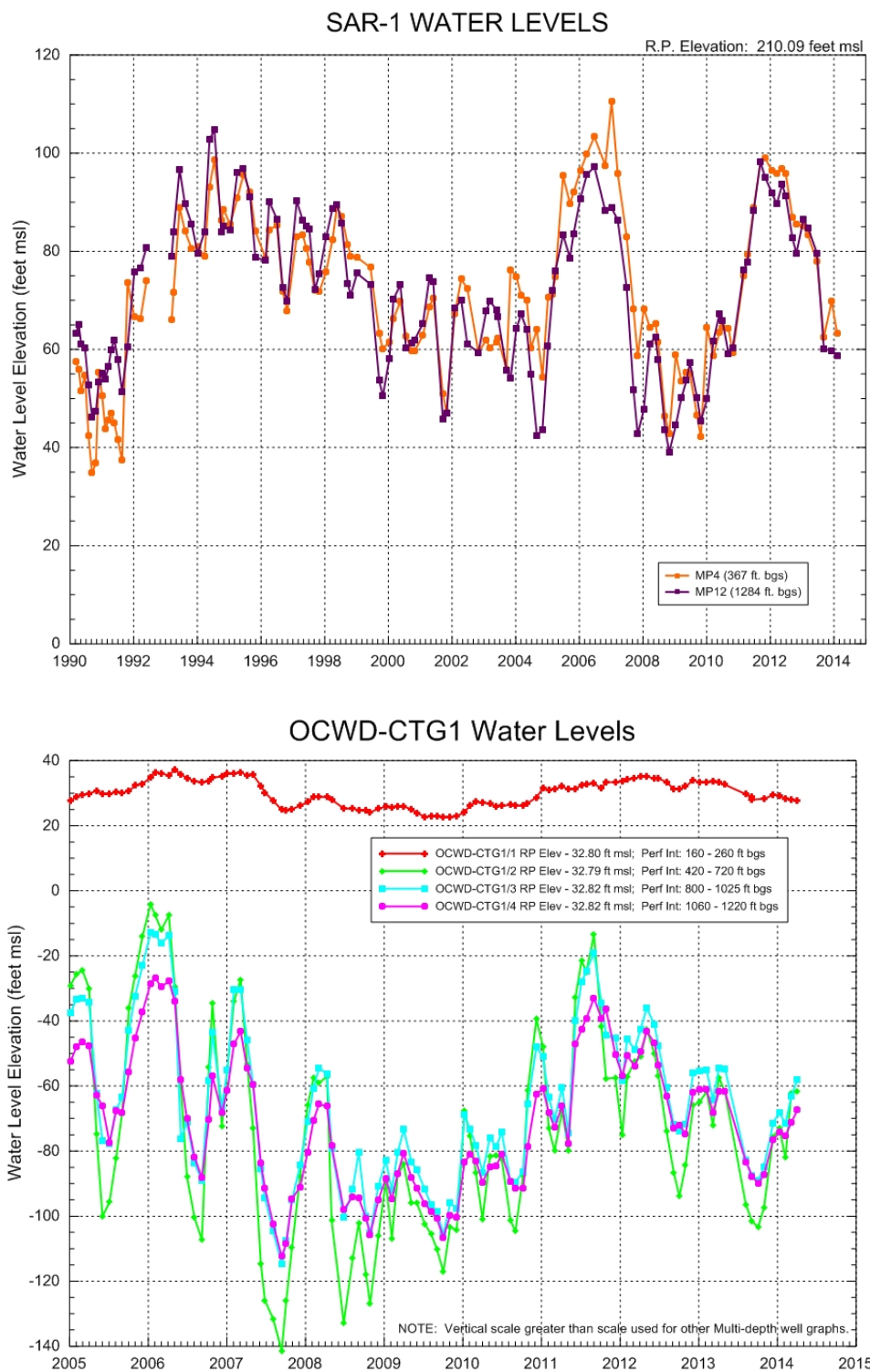
Figure 3-16: Water Level Hydrographs of Wells SAR-1 and OCWD-CTG1
