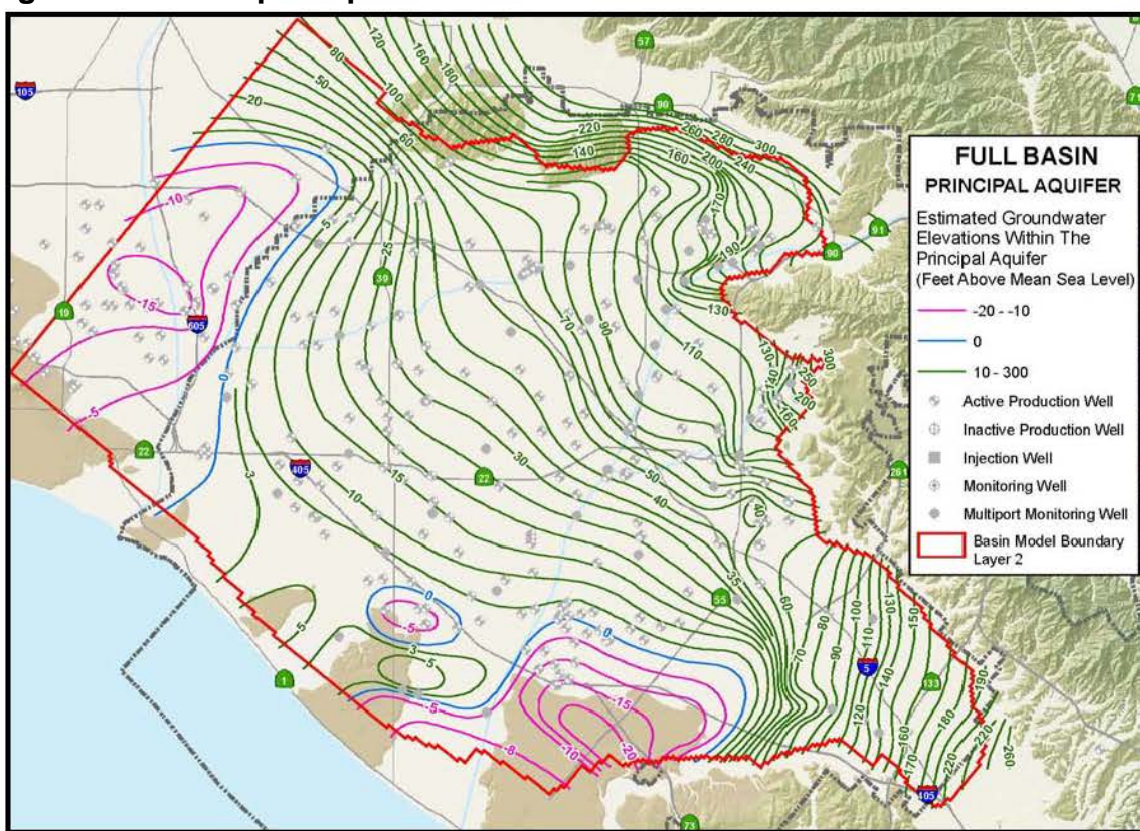
Figure 4-7. Principal Aquifer Groundwater Contours: Full Basin and June 2006
